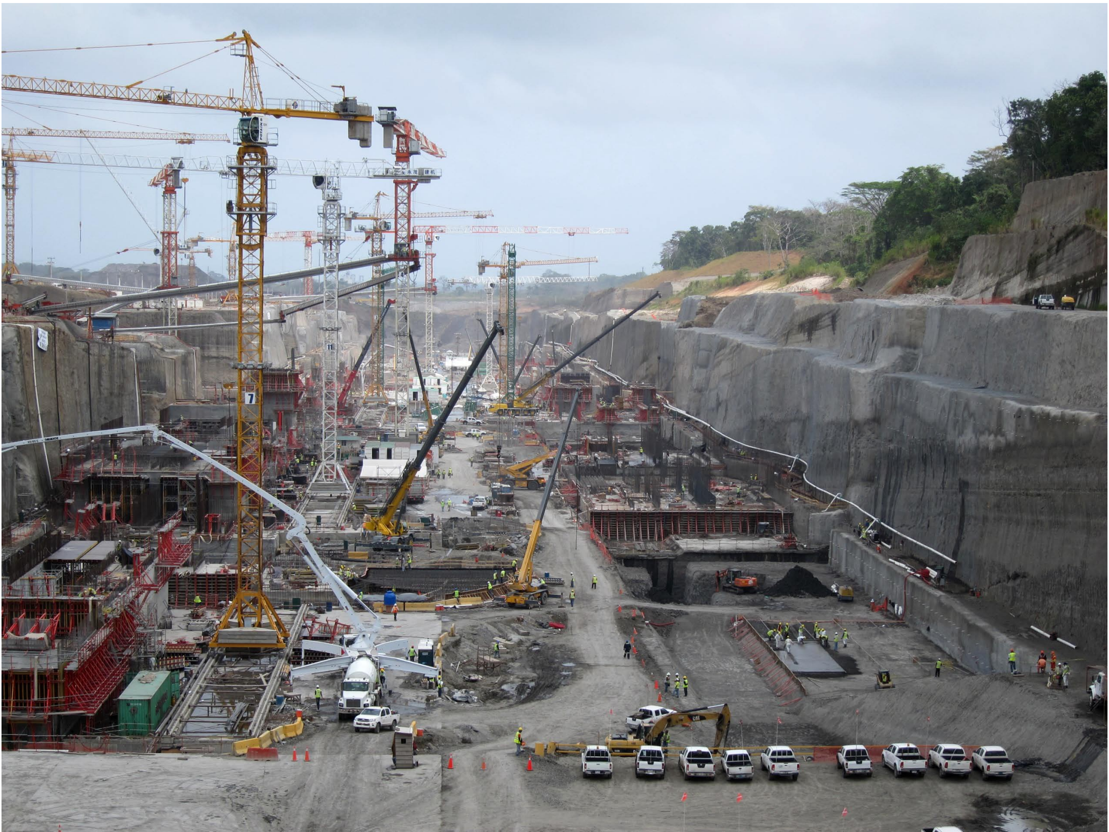
Panama Canal expansion project, Atlantic side, 2012 (Manfred Schäfer)
